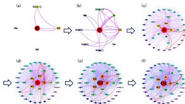
Fig. 1. Growth transition diagram to visualize the generation process of the reaction network in a He+O 2 +N 2 plasma (from (a) to (f)).
